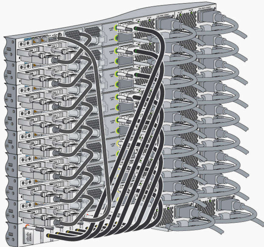
Figure 8. Cisco StackPower star topology
