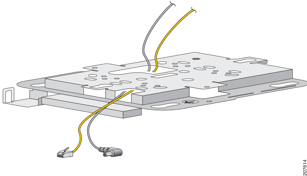
Figure 8 Routing the Ethernet and Power Cables
